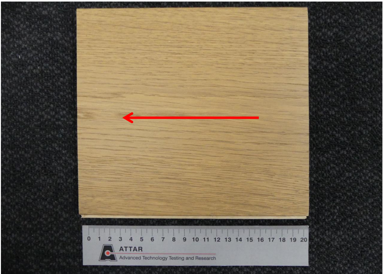
Figure 1: Wonderwood Urbana engineered timber flooring Arrow indicates direction of testing
